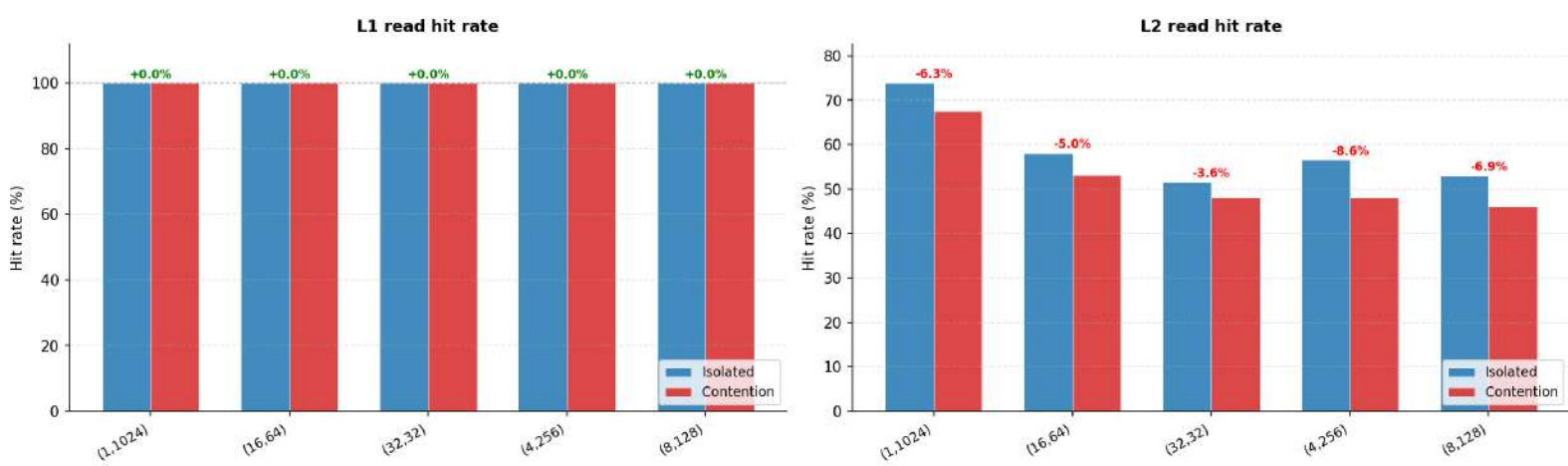
Cache hit rates: Isolated vs Contention : VectorAdd (% of accesses that hit in L1 or L2)
