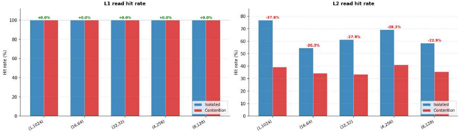
Cache hit rates: Isolated vs Contention : Convolution_2D_globalMemory (% of accesses that hit in L1 or L2)
