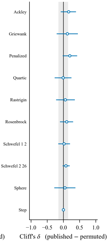
Classic F_{1..23} , 105 000 evals
