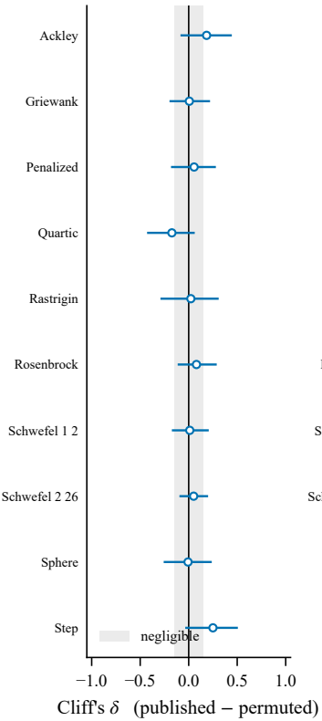
Classic F_{1..23} , 20 000 evals
