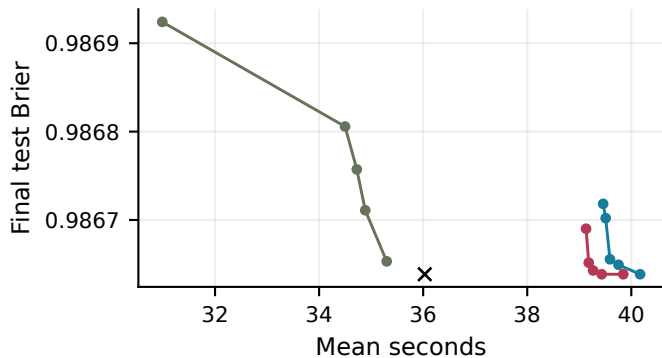
Logistic: Image-cost accounting
