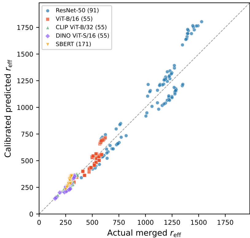
(b) Calibrated ( R^2=0.952 , MAE=48)
