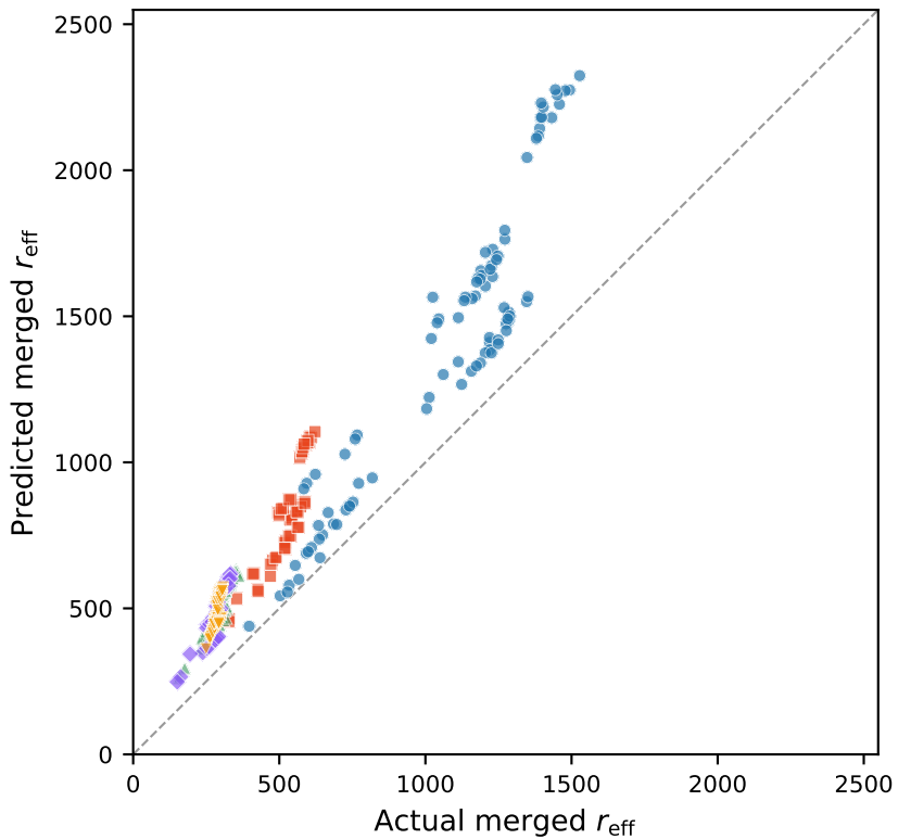
(a) Uncalibrated (Pearson r=0.970 )
