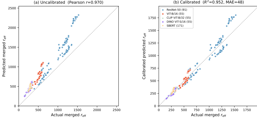
Figure 5: Predicted vs. actual merged r_{\text{eff}} for all 427 pairs across 5 encoder families. (a) Uncalibrated: formula acts as a tight upper bound (Pearson r=0.970 ). (b) After per-probe calibration: R^2=0.952 , \text{MAE}=48 . Color encodes encoder family; the identity line is dashed.
