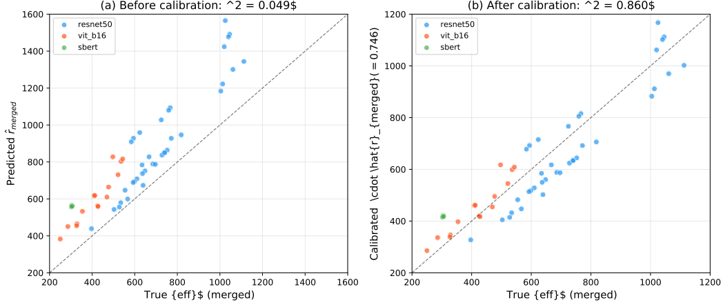
Figure 4: Elc: Predicted vs. actual merged r_{\text{eff}} for 57 real-data pairs (5 probes, 3 domain types). (a) Before calibration: systematic over-prediction ( R^2=0.049 ). (b) After single-parameter calibration ( c=0.746 ): R^2=0.860 . Pearson r=0.928 is identical in both panels—calibration corrects scale, not ranking.
