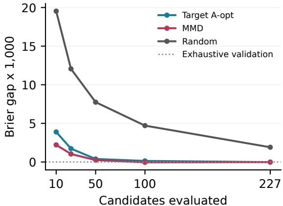
Logistic regression
