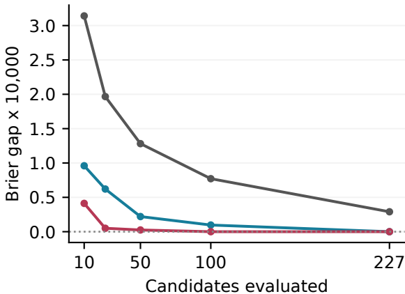
Ridge-softmax
