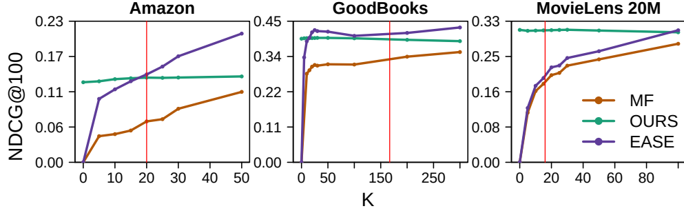
Figure A-1: NDCG@100 performance on the transition from cold-to-warm status recommendation organized by datasets.
