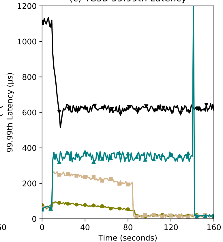
(c) YCSB 99.99th Latency
