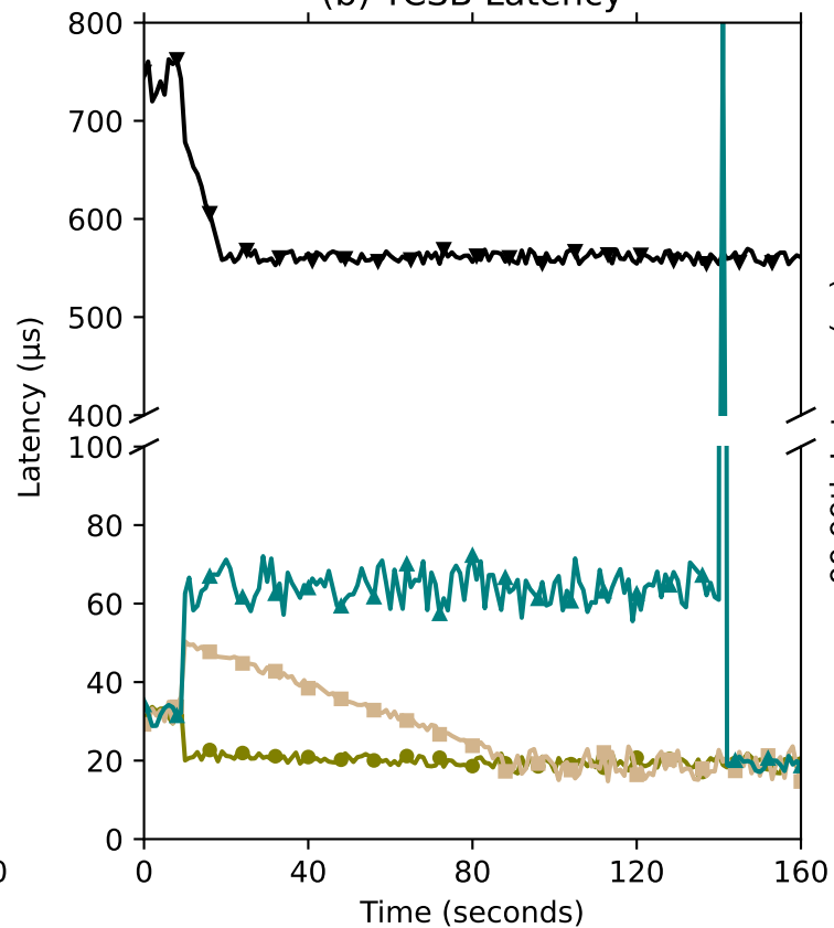
(b) YCSB Latency
