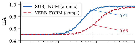
(a) Per-variable IIA (ours)
