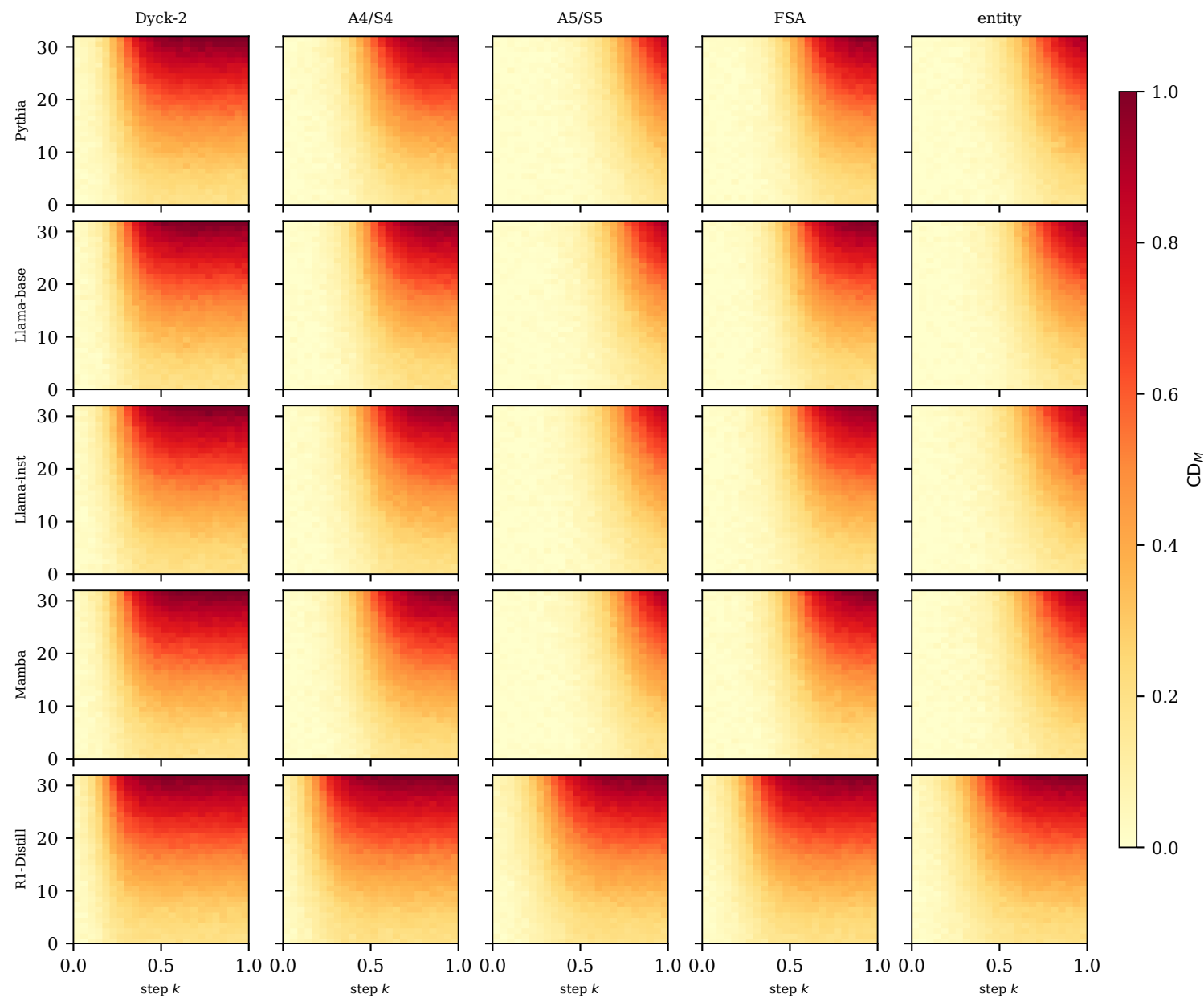
Layer ablation: CD_M(k) by layer
