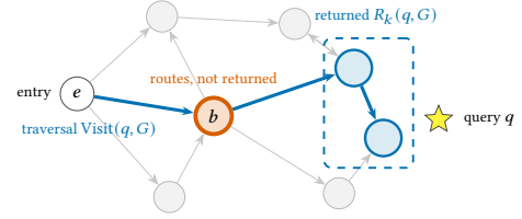
Figure 2: Greedy search for q visits the nodes on the bold path, \text{Visit}(q, G) , but returns only the k nearest, R_k(q, G) (boxed). The bridge b routes the query yet is never returned. This separation is what makes revocation subtle: once b is revoked, Tombstone filters it from R_k but leaves it routing the revoked user’s search (the zombie channel of §3), whereas LETHE routes around it. We reuse this index throughout the paper.
