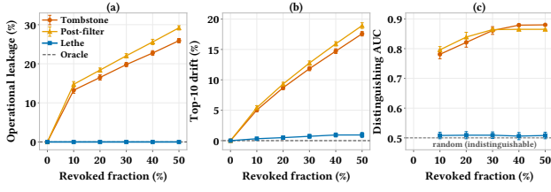
Figure 5: A revoked vector is gone from the answer and still steering the search. Result leakage is zero for every method, so a revoked vector never appears in a result and all divergence shown here is routing. (a) The fraction of traversal events that distance-score, insert into the frontier, or expand a revoked vector reaches 25.9% under Tombstone and 29.2% under Post-filter at half the index revoked, because both keep revoked vectors in the graph; LETHE encounters a revoked identifier but never scores, inserts, or expands it, so the value is identically zero and coincides with the oracle per-view rebuild. (b) The authorized top-10 consequently drifts from a truly erased index, by 17.6% (Tombstone) and 18.9% (Post-filter) at the same point, against 0.9% for LETHE . (c) A classifier given only a user’s own outputs separates a tombstoned or post-filtered index from the oracle at AUC up to 0.88 and 0.86, while LETHE stays at 0.51, on the random line. SHAREDCONFIDENTIAL , cluster revocation, four datasets, ten seeds; bars are one standard deviation.
