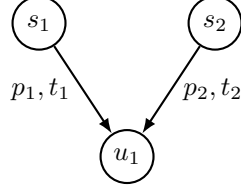
Fig. 1 Toy exposure model with two independent sources. Left: tabular representation, Right: equivalent directed graph representation.
