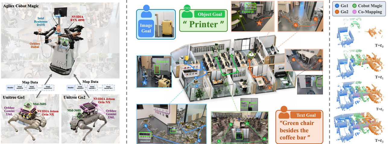
Fig. 6: Real-world deployment. Left, the three platforms—an Agilx Cobot Magic, a Unitree Go1, and a Unitree Go2—exchanging the shared map as voxel records. Center, a run with three goals—an image of a yellow suitcase, the category “printer”, and the description “green chair besides the coffee bar”—with first-person views at t_0 to t_3 ending when each robot declares its goal found. Right, the shared map growing over time, colored by robot, with regions mapped by more than one robot in pink.
