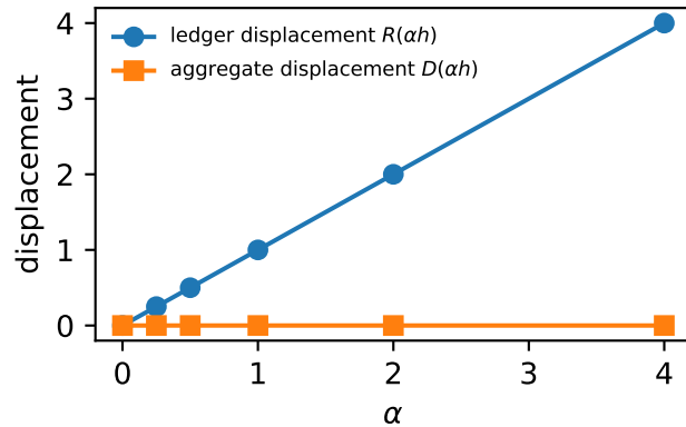
(c) Invisible fiber ( \beta = 4 )
