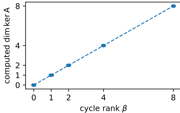
(b) Exact dimension law
