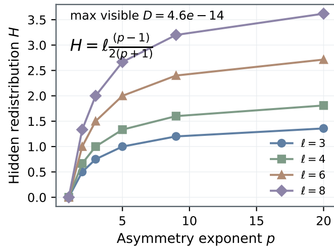
(b) Positive-complementarity cycle family
