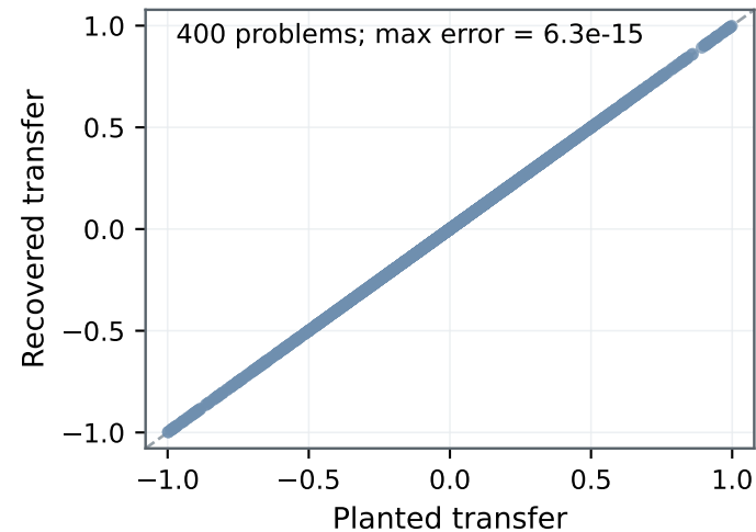
(a) Smooth realizability of prescribed transfers
