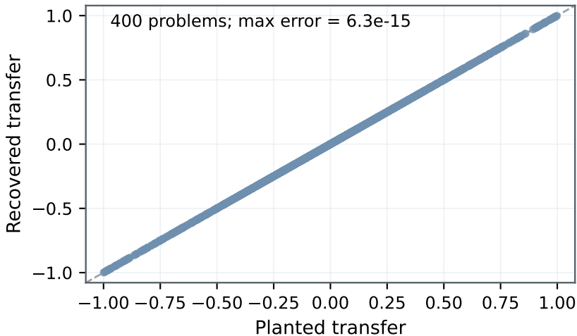
(a) Smooth realizability of prescribed transfers
