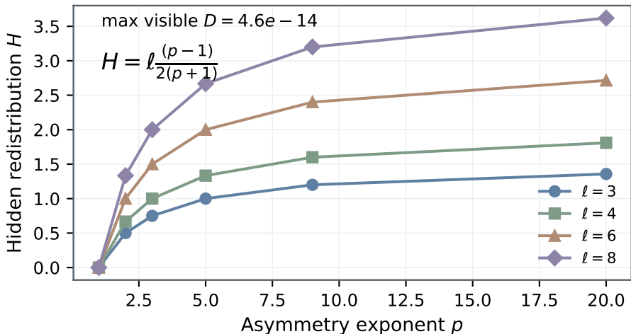
(b) Positive-complementarity cycle family
