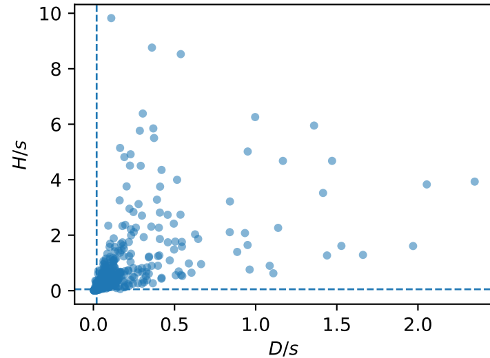
(a) CrossNet regime map
