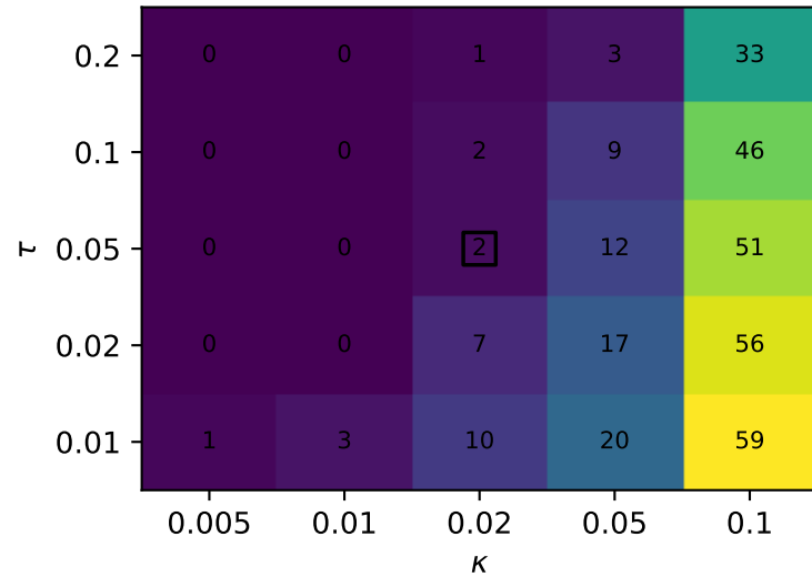
(c) Robust endpoints ( \geq 3/5 )
