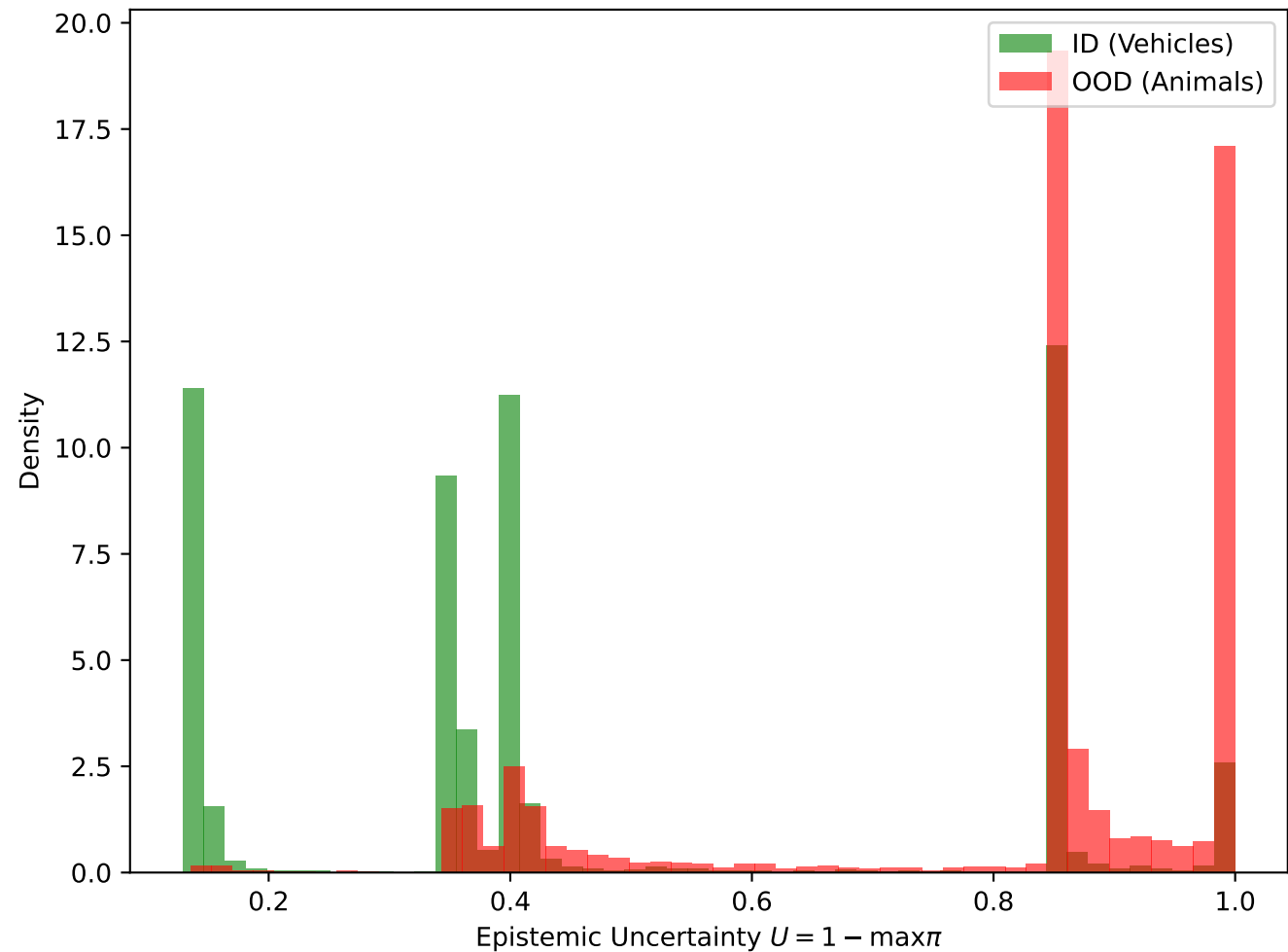
Epistemic Uncertainty Density: Joint q -Supremum
