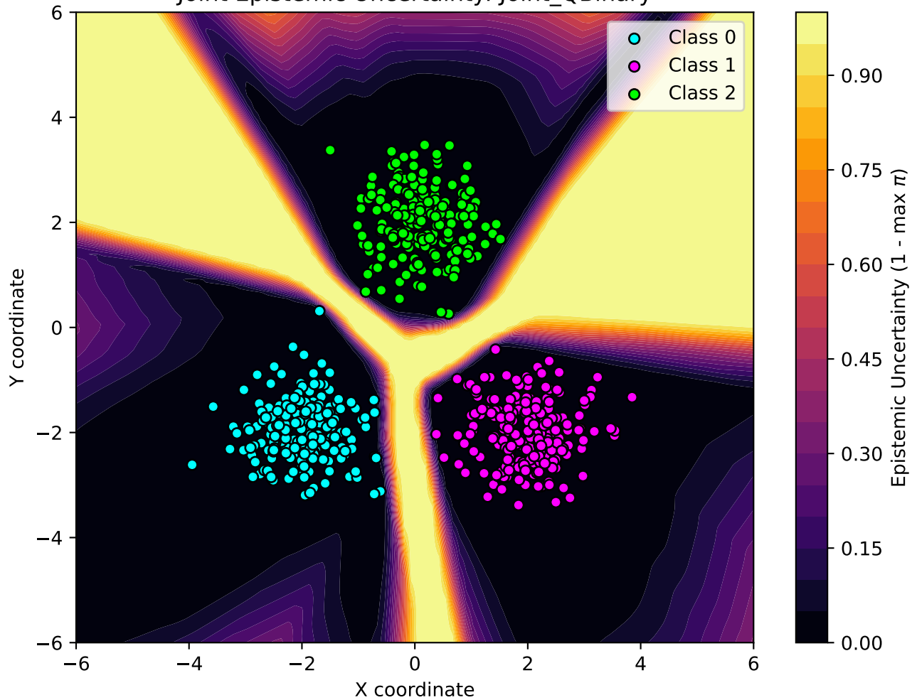
Joint Epistemic Uncertainty: Joint_QBinary
