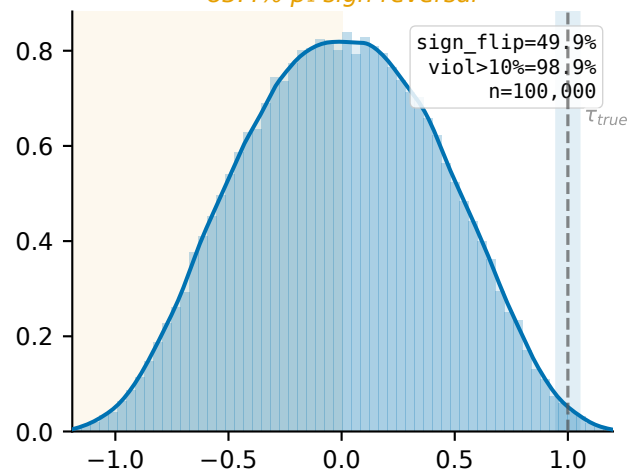
(b) Exposure
