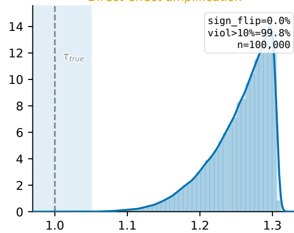
(c) Mediation
