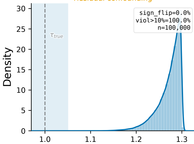
(a) Confounding
