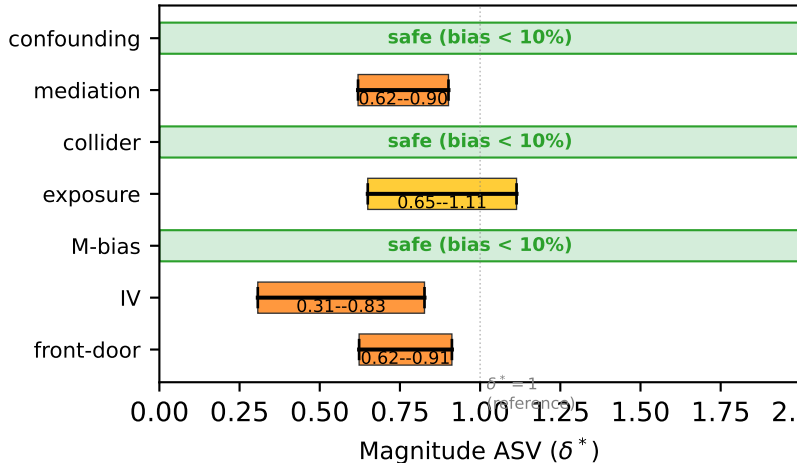
ASV Range (HumAID, K=10)
