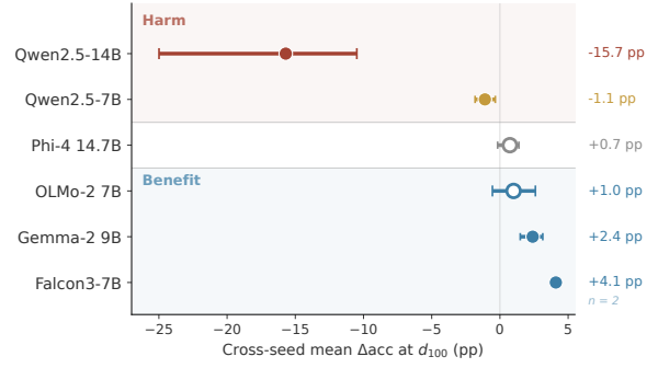
Figure 5: Cross-seed mean \Delta\text{acc} at d100 with bias-corrected and accelerated (BCa) bootstrap 95% CIs ( n = 3 seeds; Falcon3 n = 2 ). Filled markers: CI excludes zero.
