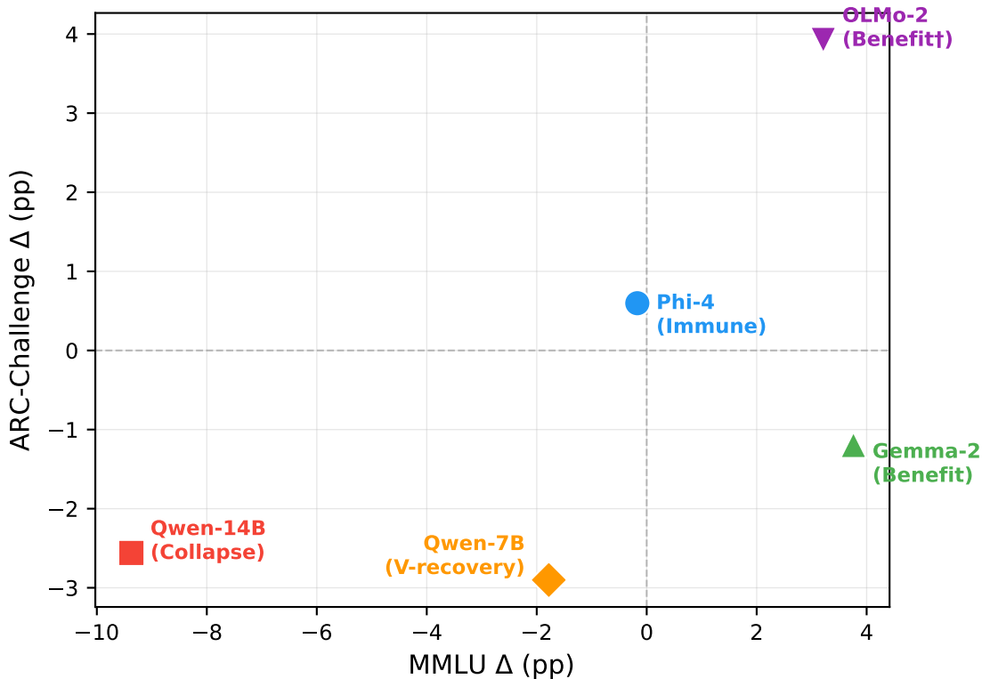
Fig. 2: Cross-benchmark scatter (seed=42; family-level taxonomy, Table 3)
