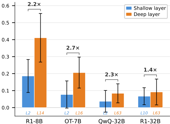
Mean step-to-step cosine distance
