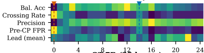
OT-7B (28 layers)
