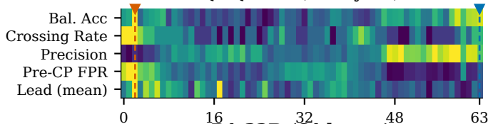
R1-32B (64 layers)
