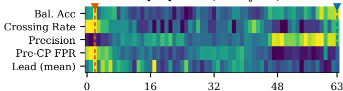
QwQ-32B (64 layers)
