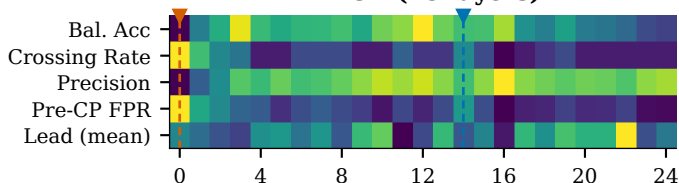
R1-8B (25 layers)
