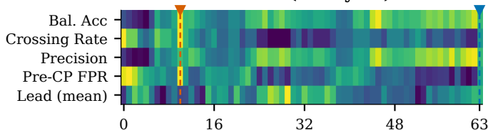
R1-32B (64 layers)
