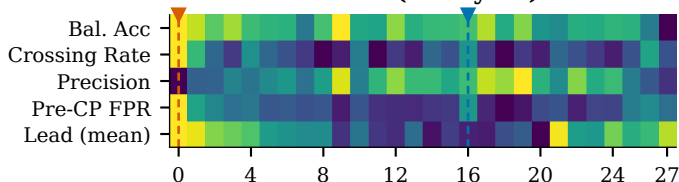
OT-7B (28 layers)
