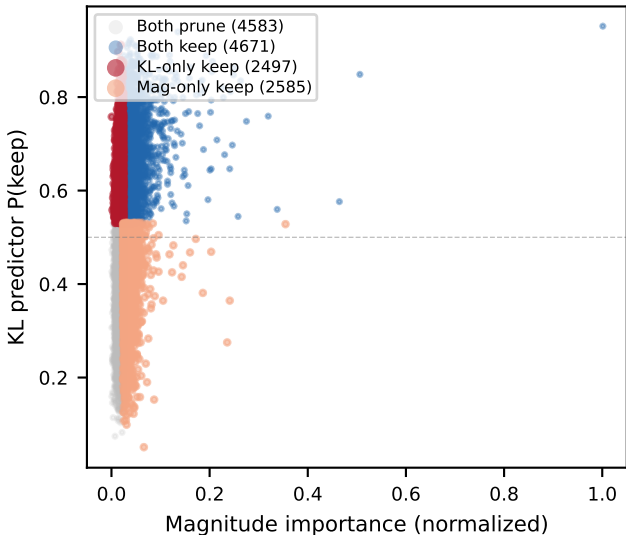
Layer 16, 50% sparsity (35.4% disagree)
