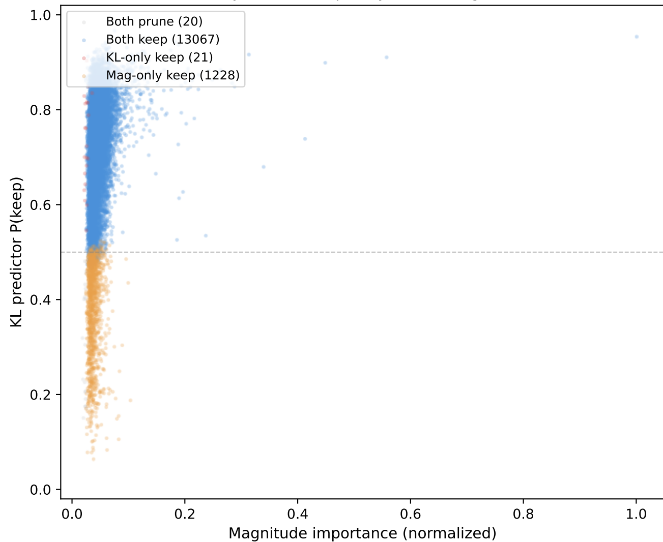
Layer 16, 30% sparsity (8.7% disagree)
