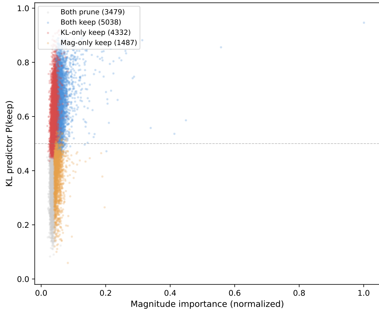
Layer 16, 50% sparsity (40.6% disagree)
