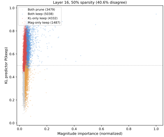
Figure 7: KL vs. magnitude importance scores for layer 16 neurons at 50% sparsity. 41% of neurons fall in disagreement quadrants where one method selects a neuron the other discards.
