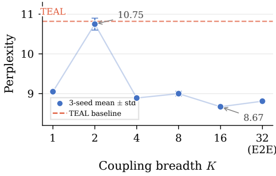
Figure 5: Coupling breadth K vs. perplexity (30%, TEAL uniform, 3-seed mean \pm std). K=32 denotes end-to-end training. K=2 degradation reflects insufficient per-layer updates ( \sim 62 vs. \sim 250 at K=8 ).
