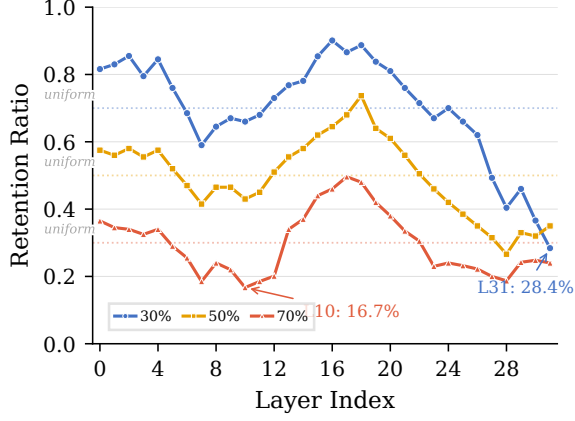
Figure 7: Per-layer neuron retention under global top- k at 30%, 50%, and 70% sparsity. Dashed lines: uniform baselines. Late layers (L24–31) are starved (28.4% at L31 even at 30%).
