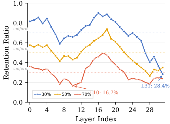
Figure 5: Per-layer neuron retention under global top- k at 30%, 50%, and 70% sparsity. Dashed lines: uniform baselines. Late layers (L24–31) are starved (28.4% at L31 even at 30%).
