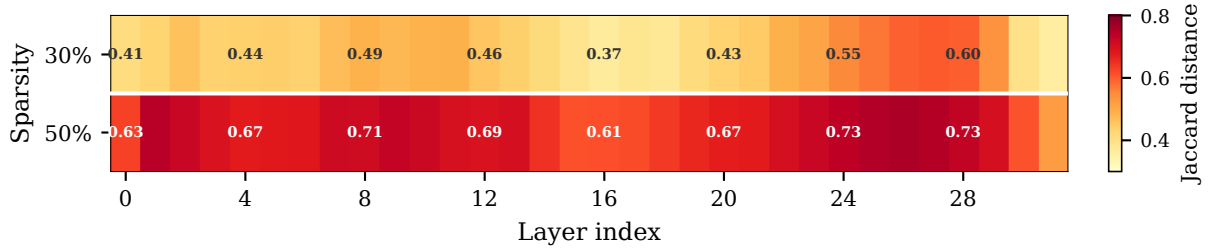
Figure 8: Per-layer Jaccard distance between KL-derived and magnitude-based masks at 30% and 50% sparsity (64 samples, 131K tokens). Divergence peaks in layers 24–28 (Jaccard distance >0.73 at 50%) and increases with sparsity across all layers.
