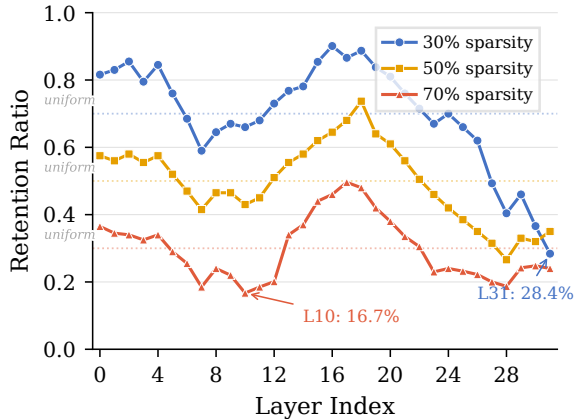
Figure 5: Per-layer neuron retention under global top- k allocation at 30%, 50%, and 70% sparsity. Dashed lines indicate uniform retention baselines. Late layers (L24–31) are consistently starved due to long-tailed activation distributions, with retention dropping to 28.4% (L31) even at 30% sparsity. At 70%, starvation extends to mid-layers (L10–12: 16.7–20.1%), explaining the transition to the capacity-limited regime.
