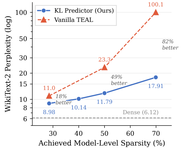
Figure 3: PPL scaling with sparsity (global allocation). KL’s advantage over TEAL grows with sparsity.
