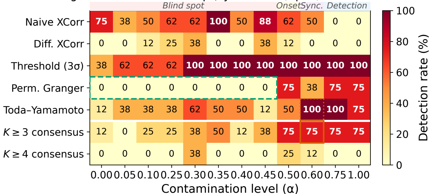
Method \times regime consensus heatmap (Pythia-410M, fp32, 12 contamination levels)
