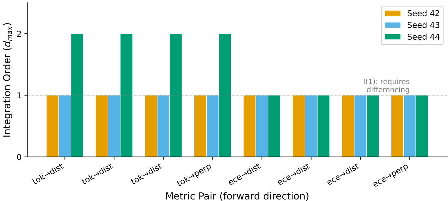
ADF Integration Order by Metric Pair ( \alpha = 0.75 )
