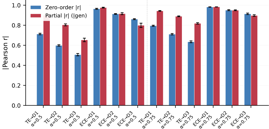
(b) Lagged (canary[t] \rightarrow downstream[t+1])
