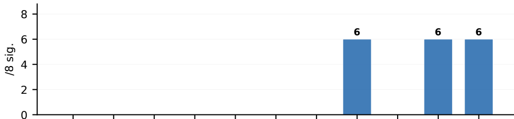
(e) Toda-Yamamoto
