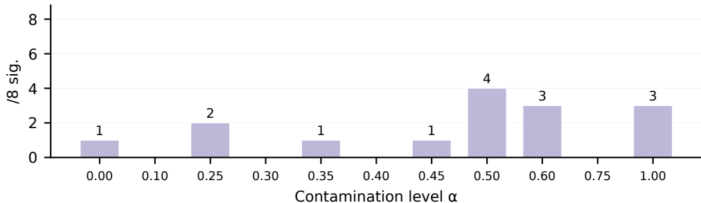
(e) Toda-Yamamoto
