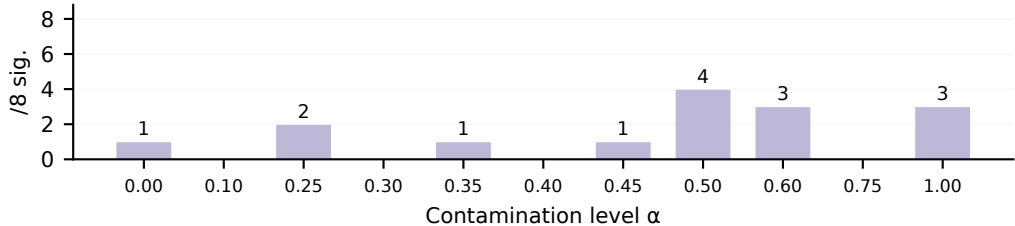
(e) Toda-Yamamoto
