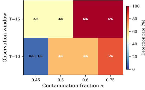
Figure 13: Pythia-1.4B phase diagram (PermG forward, 6-pair basis). Detection boundary ( \alpha_c \approx 0.50 ) is consistent with 410M.
