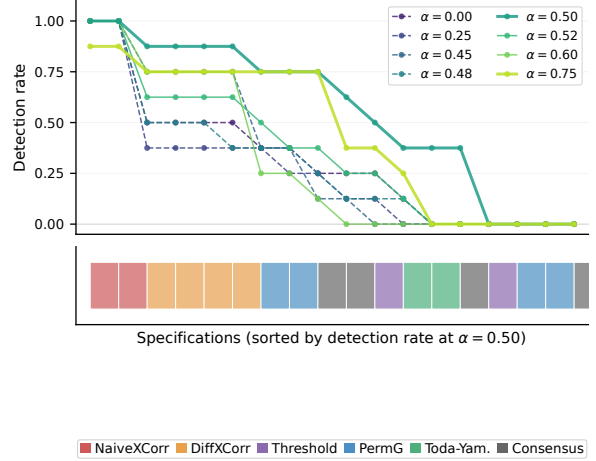
Figure 6: Specification curve (1,160 configurations). The blind \rightarrow onset jump at \alpha_c \approx 0.50 is robust across methods, pairs, and seeds.
