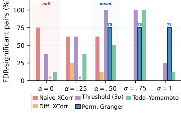
Figure 2: Method sensitivity: five methods yield dramatically different FDR-significant rates on identical data. PermG achieves the lowest null-control FPR (6.7%, pooled across 10 seeds) with 75% detection at \alpha \geq 0.50 ; dashed line: 5% nominal.
