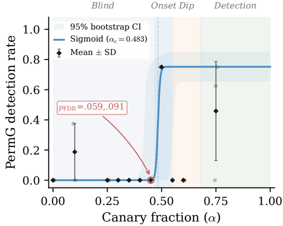
Figure 7: Dose-response: PermG detection rate with sigmoid fit ( \alpha_c=0.483 ; shaded 95% CI). Regime bands mark blind, onset, sync-dip, and detection zones.
