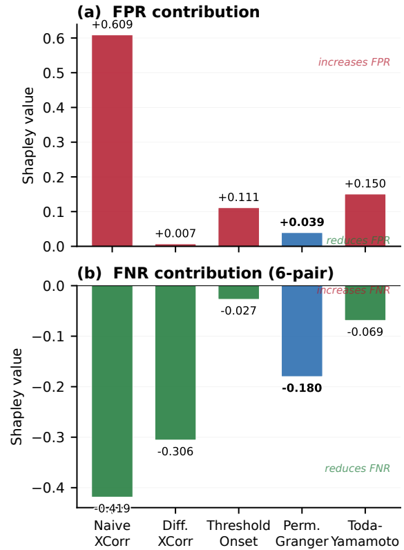
Figure 16: Shapley value decomposition by method. FPR contribution (positive = worse) and FNR contribution (negative = better) are shown for each of the five detection methods. DiffXCorr achieves the best combined Shapley ( -0.299 ) but lacks directional separation; among directional methods, PermG ranks best ( -0.141 ). NaiveXCorr contributes the most FPR ( +0.609 ) due to its inability to distinguish signal from null drift.
