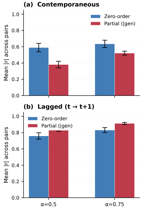
Figure 24: Aggregated partial correlation analysis across contamination levels. Lagged canary→diversity correlations increase monotonically with \alpha (from 0.524 at null to 0.913 at \alpha=0.75 ), while contemporaneous correlations plateau. The growing gap between lagged and contemporaneous partial |r| with increasing contamination indicates that the temporal lead signal strengthens with signal-to-noise ratio.
