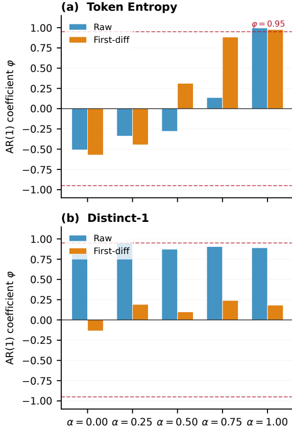
Figure 15: AR(1) coefficient estimates across five contamination levels (Pythia-410M, seed 42). (a) Token entropy: raw \phi transitions from negative ( -0.51 at \alpha=0.00 ) to near-unit-root ( 1.00 at \alpha=1.00 ), but first-differencing keeps all values below 0.98 . (b) Distinct-1: raw \phi is uniformly high ( 0.75 – 0.95 ) even at null, driven by deterministic trend; first-differencing reduces all to \leq 0.24 . Dashed red line: \phi=0.95 danger zone.
