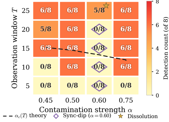
Figure 1: Phase diagram (Pythia-410M, fp32, PermG). FDR-significant canary→diversity pairs across \alpha and T ; dashed curve: fitted boundary (Eq. 1); ◇: non-monotonic anomaly; ★: dissolution at T=25 .
