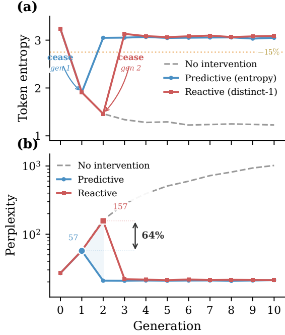
Figure 9: Canary-triggered intervention (Pythia-410M, \alpha=1.0 ). Predictive cessation on entropy (generation 1) reduces peak perplexity by 64% versus reactive triggering on distinct-1 (generation 2).
