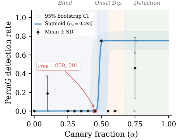
Figure 4: Dose-response: PermG detection rate with sigmoid fit ( \alpha_c=0.483 ; shaded 95% CI). Regime bands mark blind, onset, sync-dip, and detection zones.
