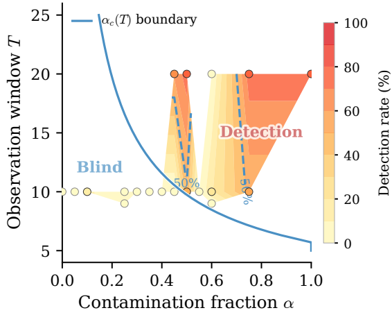
Figure 24: Detection rate surface over \alpha \times T (PermG forward, 3 seeds). Dashed curve: fitted boundary \alpha_c(T) . The blind zone ( \alpha \leq 0.45 ) shrinks as T increases.
