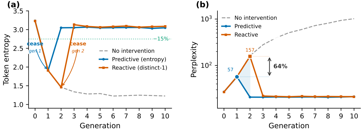
Figure 6: Canary-triggered intervention (Pythia-410M, \alpha=1.0 ). Predictive cessation on entropy (generation 1) reduces peak perplexity by 64% versus reactive triggering on distinct-1 (generation 2).
