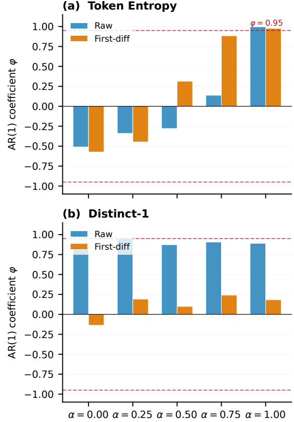
Figure 13: AR(1) coefficient estimates across five contamination levels (Pythia-410M, seed 42). (a) Token entropy: raw \phi transitions from negative ( -0.51 at \alpha=0.00 ) to near-unit-root ( 1.00 at \alpha=1.00 ), but first-differencing keeps all values below 0.98. (b) Distinct-1: raw \phi is uniformly high ( 0.75 – 0.95 ) even at null, driven by deterministic trend; first-differencing reduces all to \leq 0.24 . Dashed red line: \phi=0.95 danger zone.
