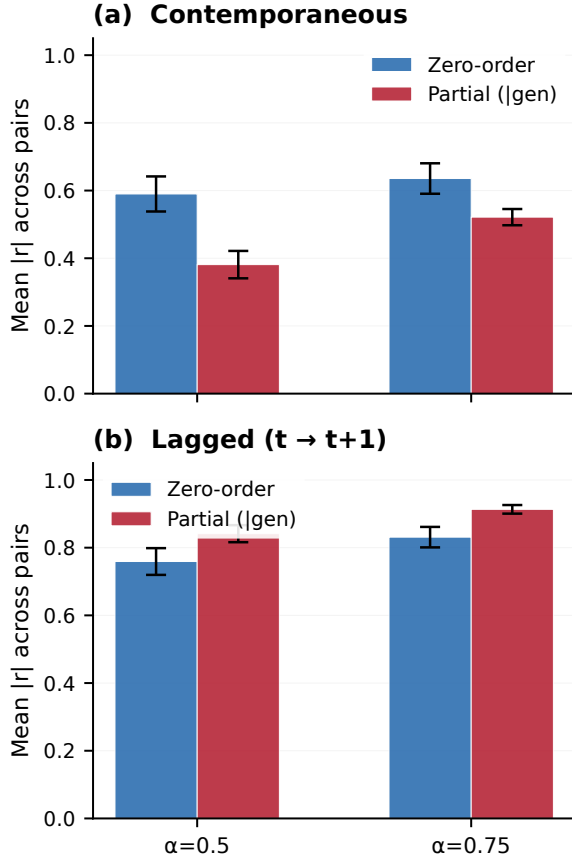
Figure 22: Aggregated partial correlation analysis across contamination levels. Lagged canary \rightarrow diversity correlations increase monotonically with \alpha (from 0.524 at null to 0.913 at \alpha=0.75 ), while contemporaneous correlations plateau. The growing gap between lagged and contemporaneous partial |r| with increasing contamination indicates that the temporal lead signal strengthens with signal-to-noise ratio.
