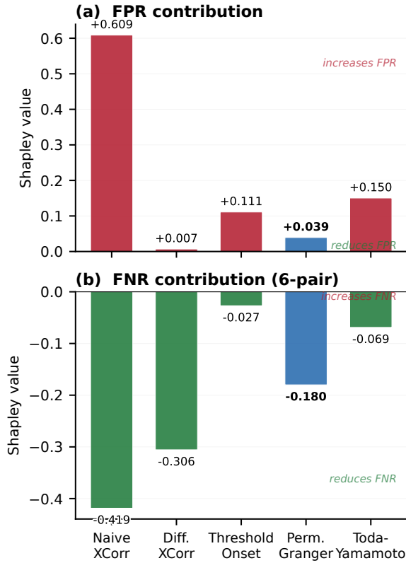
Figure 14: Shapley value decomposition by method. FPR contribution (positive = worse) and FNR contribution (negative = better) are shown for each of the five detection methods. DiffXCorr achieves the best combined Shapley ( -0.299 ) but lacks directional separation; among directional methods, PermG ranks best ( -0.141 ). NaiveXCorr contributes the most FPR ( +0.609 ) due to its inability to distinguish signal from null drift.
