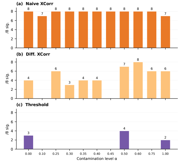
Figure 12: Per-method FDR-significant pair counts (/8) across contamination levels (Pythia-410M, seed 42, T=10 , fp32). PermG (d) exhibits the cleanest regime separation—zero detections through \alpha=0.45 , then a steep 0→6 jump at \alpha=0.50 ; NaiveXCorr (a) saturates at 7–8/8 across all levels including null; DiffXCorr (b) detects signal but cannot separate forward from reverse. The visual contrast across panels illustrates why method choice is itself a primary source of variability ( \kappa=0.187 ).
