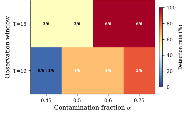
Figure 11: Pythia-1.4B phase diagram (PermG forward, 6-pair basis). Detection boundary ( \alpha_c \approx 0.50 ) is consistent with 410M.
