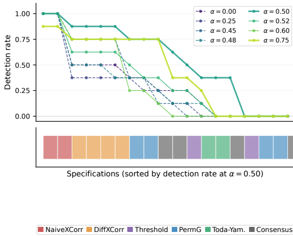
Figure 8: Specification curve (288 configurations). The blind \rightarrow onset jump at \alpha_c \approx 0.50 is robust across methods, pairs, and seeds.
