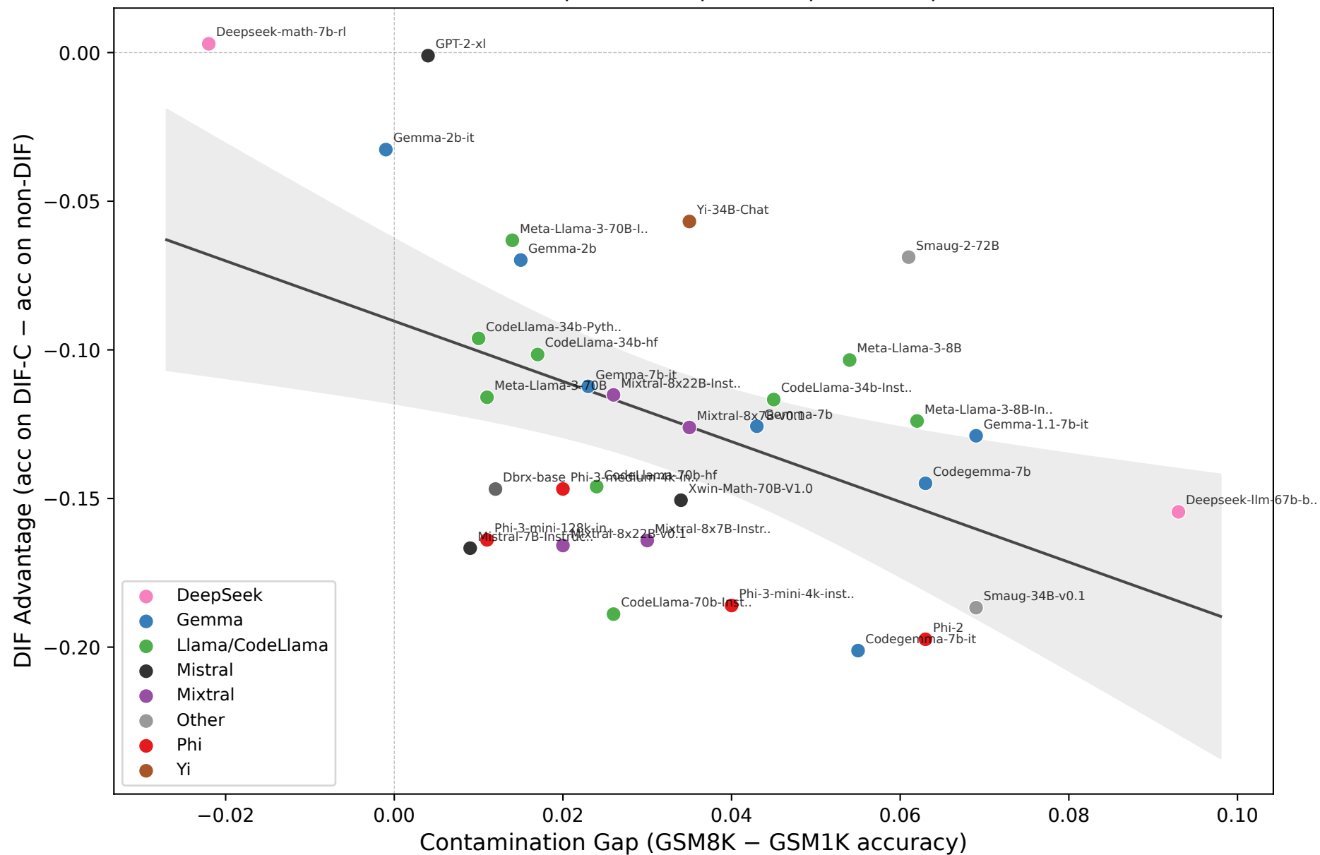
GSM1K Contamination Gap vs. DIF-C Item Advantage Pearson r=-0.478 ( p=0.005 ), Spearman \rho=-0.403 ( p=0.020 )
