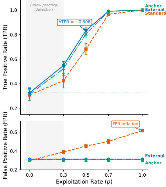
Figure 3: Semi-synthetic dose-response for DIF detection on MMLU. \Delta\text{TPR} ( = \text{TPR}_{\text{injected}} - \text{TPR}_{\text{baseline}} ) increases monotonically with exploitation rate p under binary injection (a calibration upper bound; Section 3.4); MH-DIF is sensitive to differential item behavior when present. Baseline (no injection) produces \Delta\text{TPR} \approx 0 .
