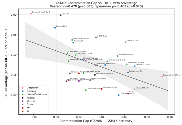
Figure 7: Exploratory: GSM1K contamination gap vs. DIF ranking advantage ( N = 33 ; small sample, results should be interpreted cautiously). The negative correlation ( r = -0.478 , p = 0.005 ) indicates that models with larger contamination gaps benefit less from DIF-flagged items. Three of 33 models exceed the Cook’s D threshold ( 4/N = 0.12 ); leave-one-out analysis confirms all individual-removal correlations remain significant ( r \in [-0.54, -0.37] , all p < 0.05 ), and removing all three outliers yields r = -0.38 ( p = 0.036 , N = 30 ).
