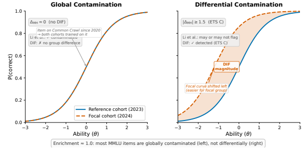
Figure 2: Global vs. differential contamination via Item Characteristic Curves (ICCs). Left: global contamination produces no DIF; both cohorts encounter the item, and their ICCs overlap. Right: differential contamination produces DIF; the focal cohort’s ICC shifts due to disproportionate exposure. The enrichment ratio of \approx 1.0 between DIF flags and web-overlap labels is expected because most items fall into the left category.
