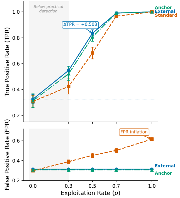
Figure 2: Semi-synthetic dose-response for DIF detection on MMLU. \Delta TPR (= TPR_{\text{injected}} - TPR_{\text{baseline}}) increases monotonically with exploitation rate p under binary injection (a calibration upper bound; Section 3.4); MH-DIF is sensitive to differential item behavior when present. Baseline (no injection) produces \Delta TPR \approx 0 .
