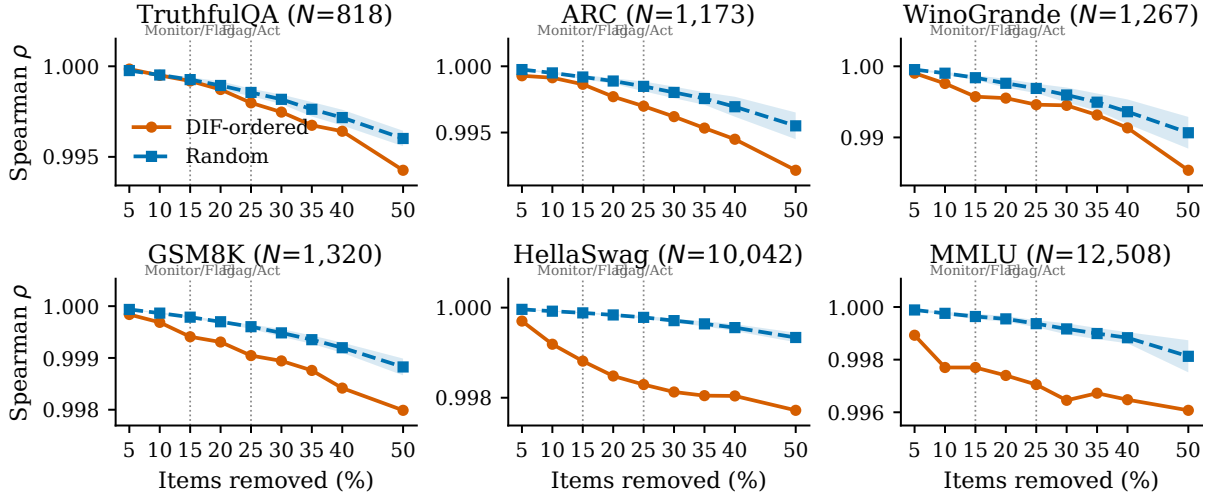
Figure 3: Ranking degradation under DIF-ordered vs. random item removal. DIF-ordered removal (orange) degrades \rho faster than random (blue band = mean \pm 1 SD, 20 seeds). Dashed lines: Monitor/Flag (15%) and Flag/Act (25%) thresholds (Section 5.2).
