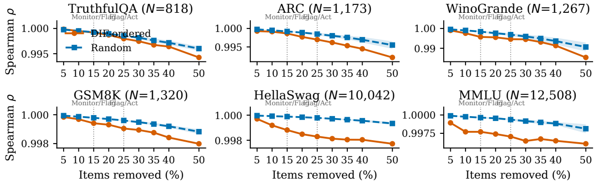
Figure 3: Ranking degradation under DIF-ordered vs. random item removal. DIF-ordered removal (orange) degrades \rho faster than random (blue band = mean \pm 1 SD, 20 seeds). Dashed lines: Monitor/Flag (15%) and Flag/Act (25%) thresholds (Section 5.2).
