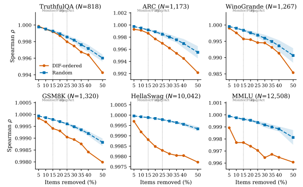
Figure 6: Ranking degradation under DIF-ordered vs. random item removal across six benchmarks. DIF-ordered removal (red) consistently degrades \rho faster than random removal (blue band = mean \pm 1 SD, 20 seeds). Vertical dashed lines mark the Monitor/Flag (15%) and Flag/Act (25%) thresholds from Section 5.3.
