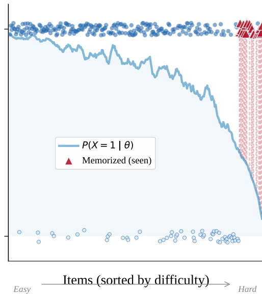
(b) Contaminated Model
